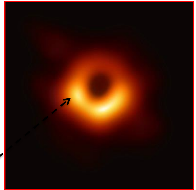
Direct image of a supermassive black hole at the core of Messier 87.
