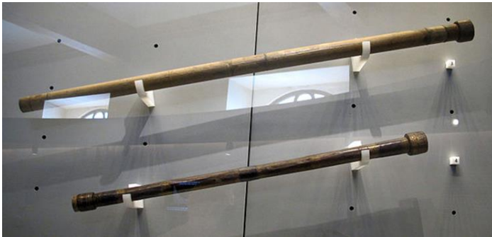
Galileo's telescopes. Credit: Sailko/CC BY-SA 3.0
